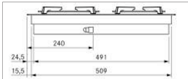
Fig. 3.31 PKG3 appliance dimensions side view
